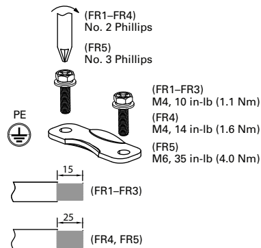
Figure 25. Grounding
