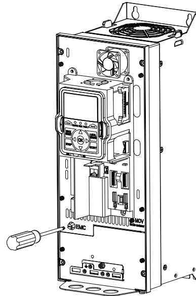
Figure 30. Locations of the EMC Screws in Frame 5
