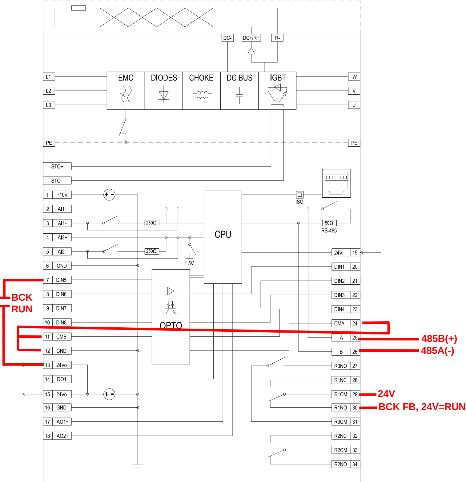
Figure 21. Basic Internal Control Wiring Diagram
