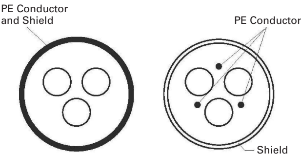
Figure 28. Cable Description
