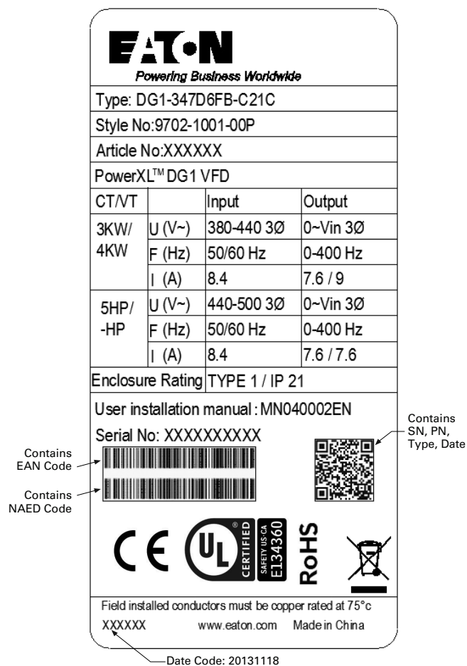
Figure 2. Rating Label
