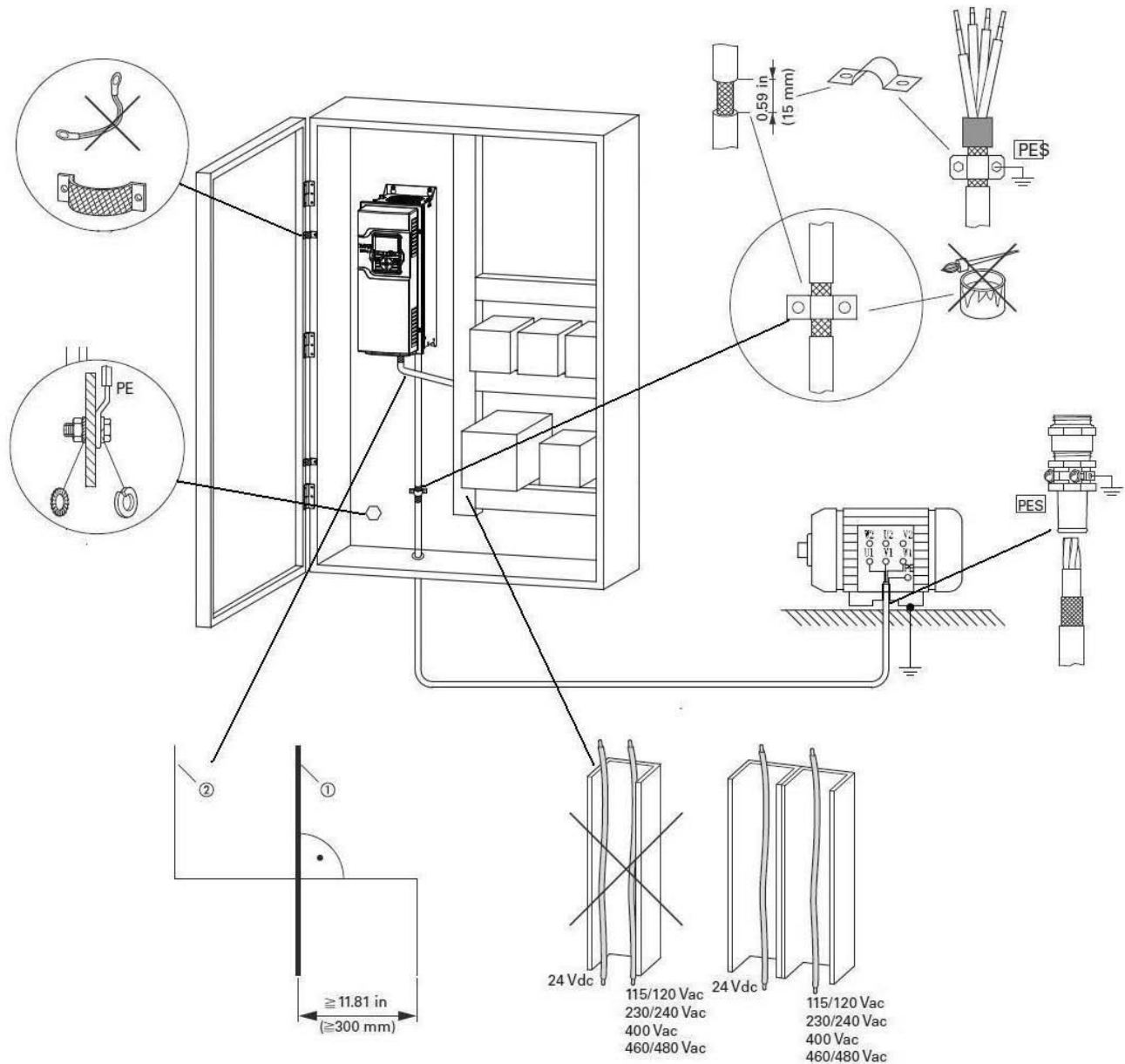
Figure 27. EMC-Compliant Setup—460/480 Vac
