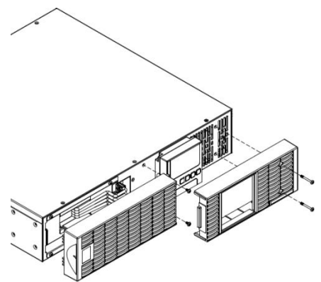
Step 5: Install the front panels
