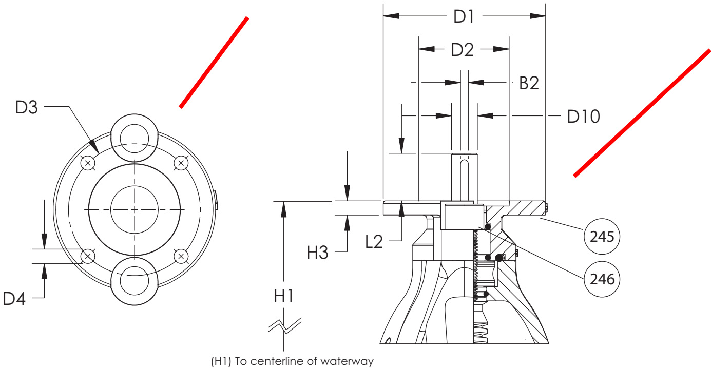
(H1) To centerline of waterway
